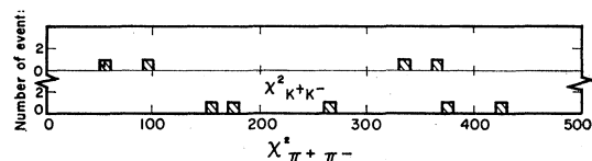
FIG. 3. Histograms of the \chi^2 distribution for the \pi^+\pi^- and K^+K^- hypotheses for the simulated events. Each event is plotted only once.
