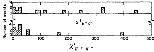
FIG. 2. Histograms of the \chi^2 distribution for the \pi^+\pi^- and K^+K^- hypotheses for events from the random sample of two prongs. Each event is plotted only once.
