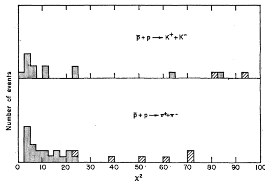
FIG. 1. Histograms of the \chi^2 distribution for the selected sample of two-prong events for the hypotheses of \bar{p}+p \rightarrow \pi^+\pi^- and \bar{p}+p \rightarrow K^+K^- . Some events occur on both plots. The cross-hatched squares represent events that have a smaller \chi^2 for the other two-meson interpretation.
