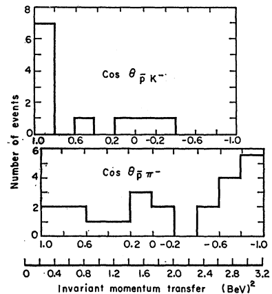
FIG. 4. Histograms of the distribution of the c.m. angle for the events that fit the \pi^+\pi^- and K^+K^- hypotheses. The distributions are plotted in such a way that one can directly compare the differential cross sections d\sigma/dS as a function of momentum transfer.
